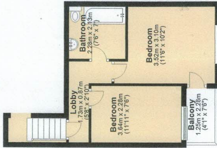
Third Floor Approx. 31.5 sq. metres (338.9 sq. feet)
